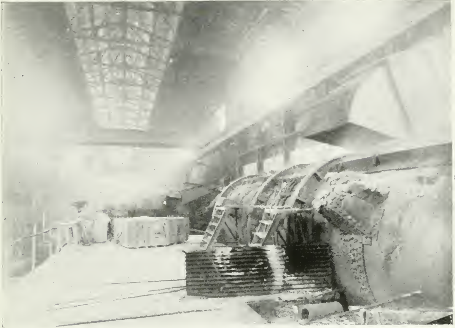
Fig. 72—Interior of Converter Building, Canadian Copper Company, Copper Cliff, Ontario.
